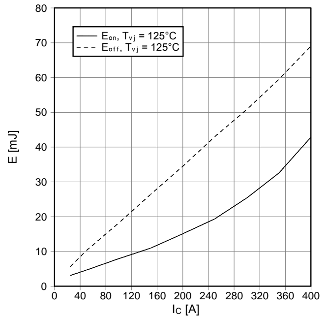
Schaltverluste IGBT-Wechselr. (typisch) switching losses IGBT-inverter (typical) E_{on} = f(I_c), E_{off} = f(I_c) V_{GE} = \pm 15\text{ V}, R_{Gon} = 3,6\ \Omega, R_{Goff} = 3,6\ \Omega, V_{CE} = 600\text{ V}
