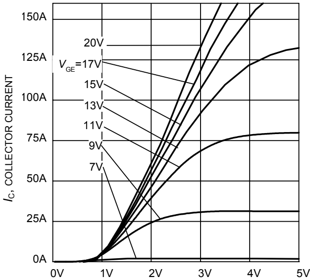
Figure 5. Typical output characteristic ( T_j = 25^\circ\text{C} )
