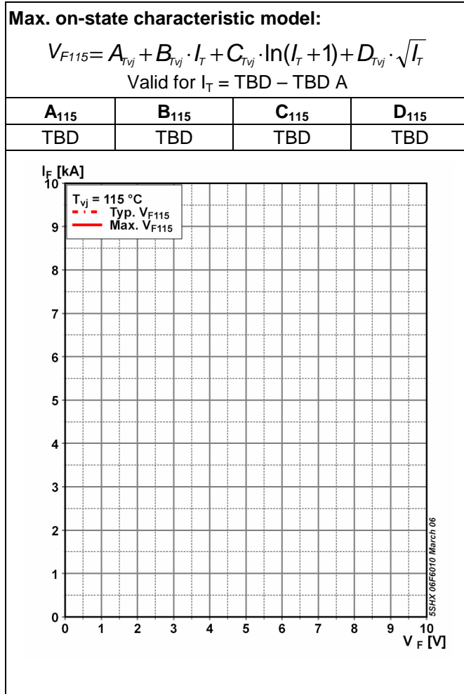
Fig. 10 Diode on-state voltage characteristics
