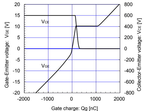
Dynamic Gate Charge (typ.) V CC =600V, I c =200A, T j = 25°C
