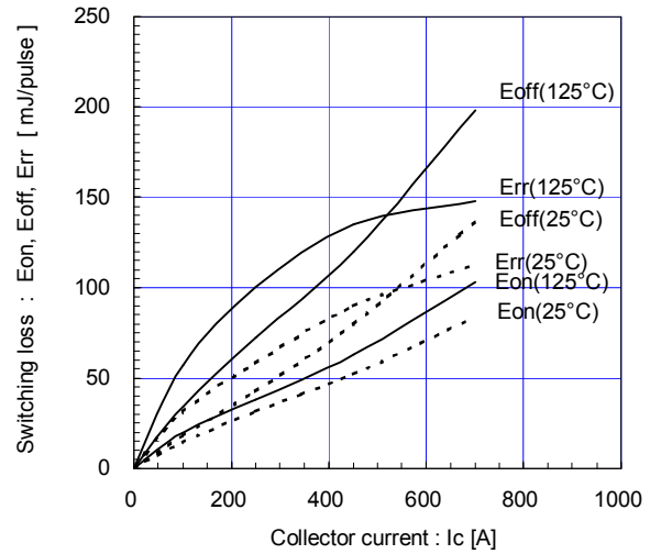
Switching loss vs. Collector current (typ.) V_{cc}=900V, V_{GE}=\pm 15V, R_g=1.1\Omega
