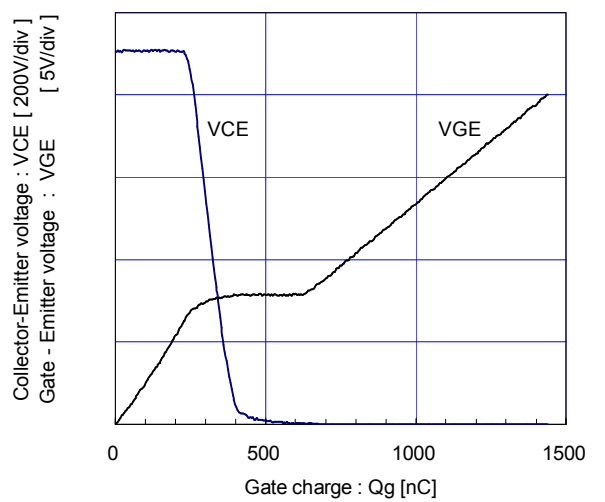
Dynamic Gate charge (typ.) Vcc=900V, Ic=450A, Tj= 25°C
