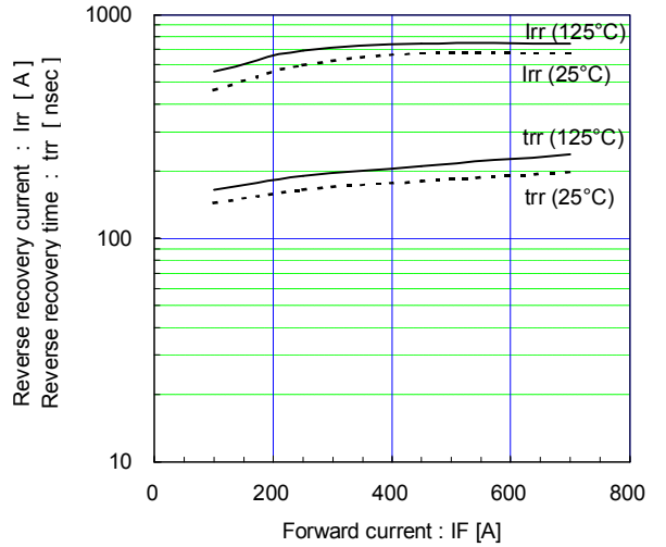
Reverse recovery characteristics (typ.) Vcc=900V, VGE=±15V, Rg=1.1Ω
